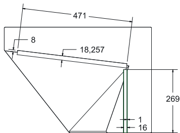
SECTION A-A Wireway and LED light niche
