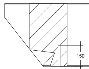
SECTION B-B Fixing into the ground
